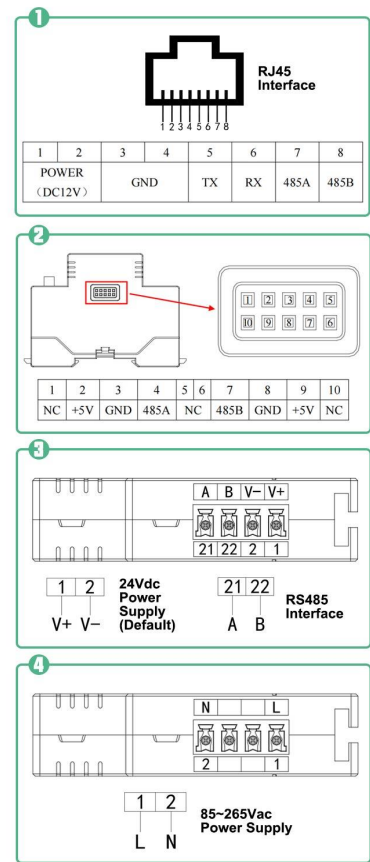
PIN Overview of AWT100-WiFiHW
